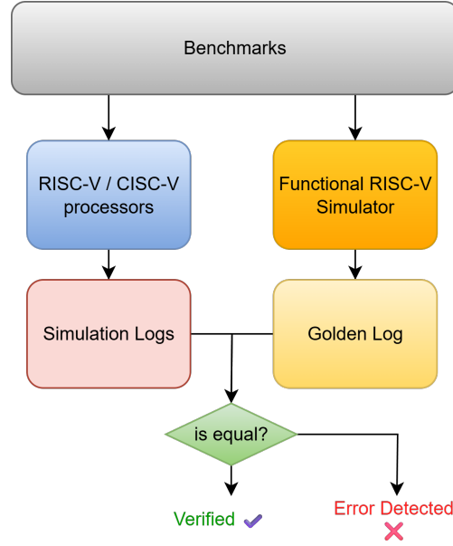
Figure 8: Log-based Verification Framework
